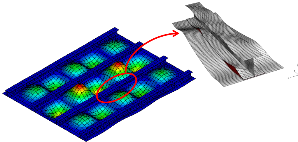
Figure 2: A postbuckling stiffened composite panel showing localised skin-stiffener separation.
