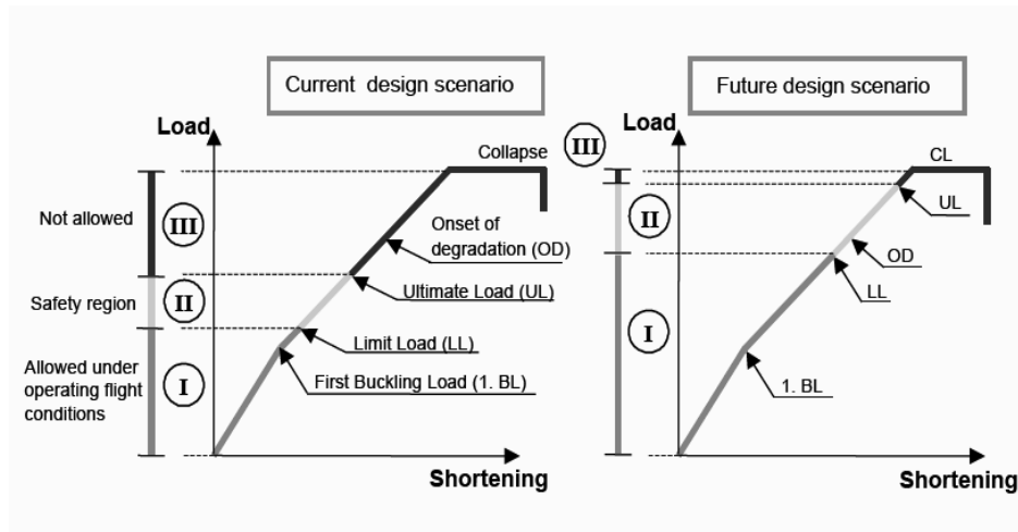
Figure 1: Composites design philosophy; (a) current and (b) future design scenarios. [courtesy of DLR].
